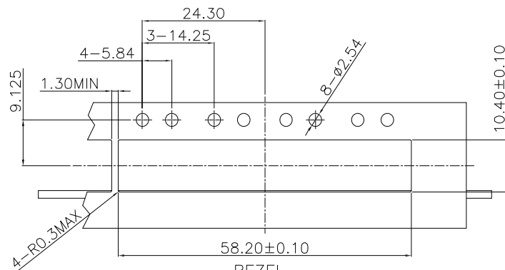
BEZEL RECOMMENDED PANEL CUTOUT AND PC BOARD PANEL POSITION AND THICKNESS 0.8-2.6
