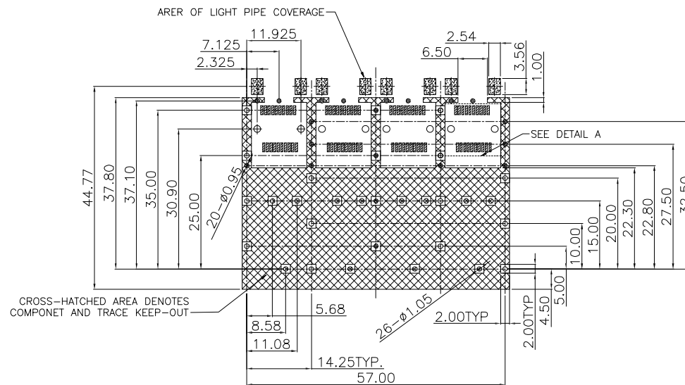
BEZEL RECOMMENDED PANEL CUTOUT AND PC BOARD PANEL POSITION AND THICKNESS 0.8-2.6
