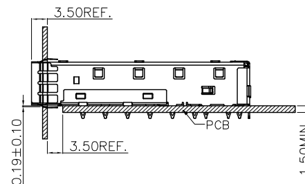
BEZEL OPENING BELOW TOP OF PCB
