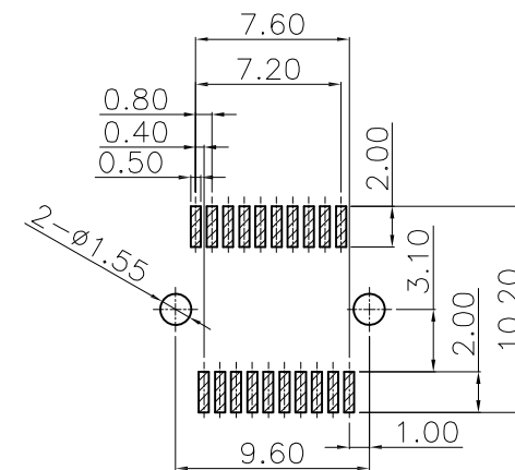
DETAIL A(SCALE 2:1)
