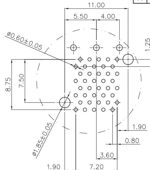
DETAIL A(SCALE 2:1)
