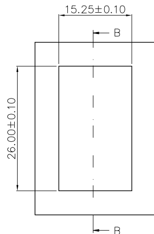
BEZEL CUT-OUT OPENING DETAIL
