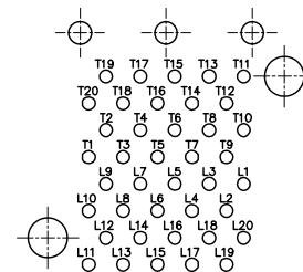
CONNETTON PINOUT DETAIL COMPONENT SIDE OF BOARD
