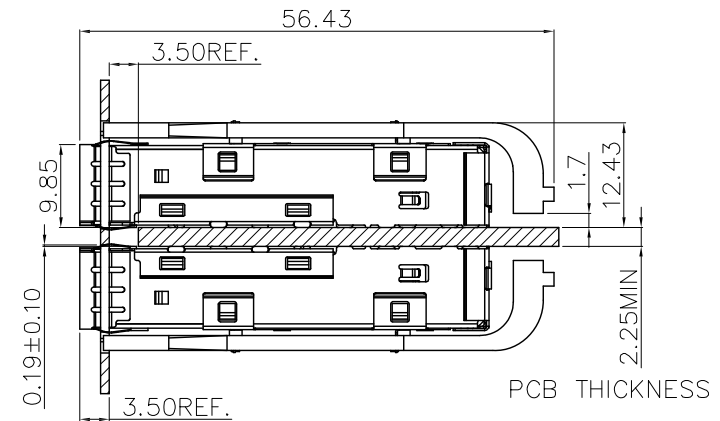
BEZEL OPENING BELOW TOP OF PCB
