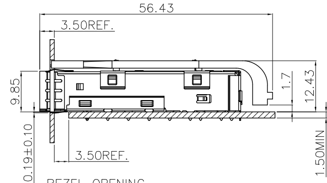
BEZEL OPENING BELOW TOP OF PCB
